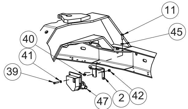
WATER VALVE INSTALL DETAIL
